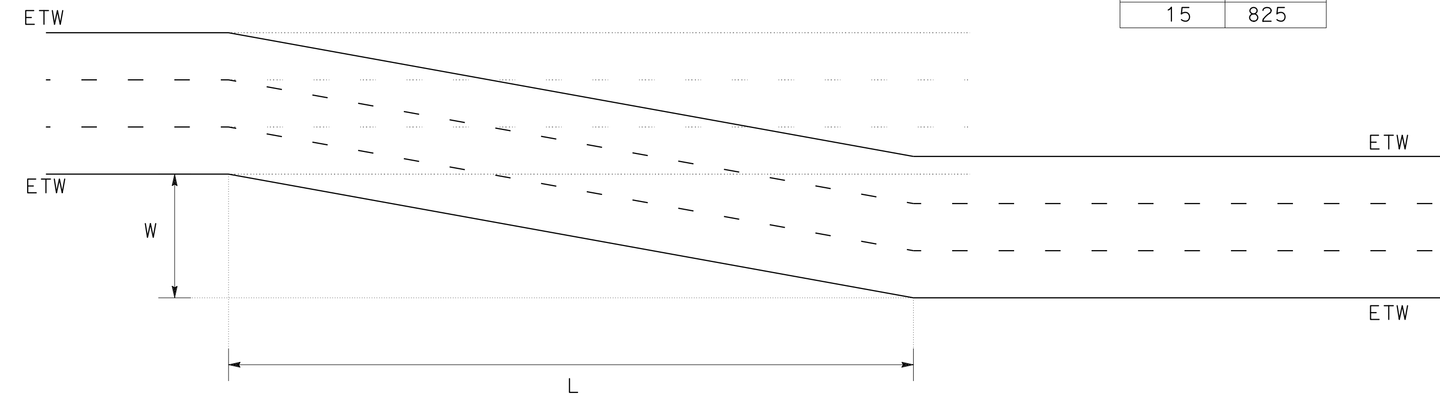
LANE TRANSITION TAPER LENGTH DETAIL
