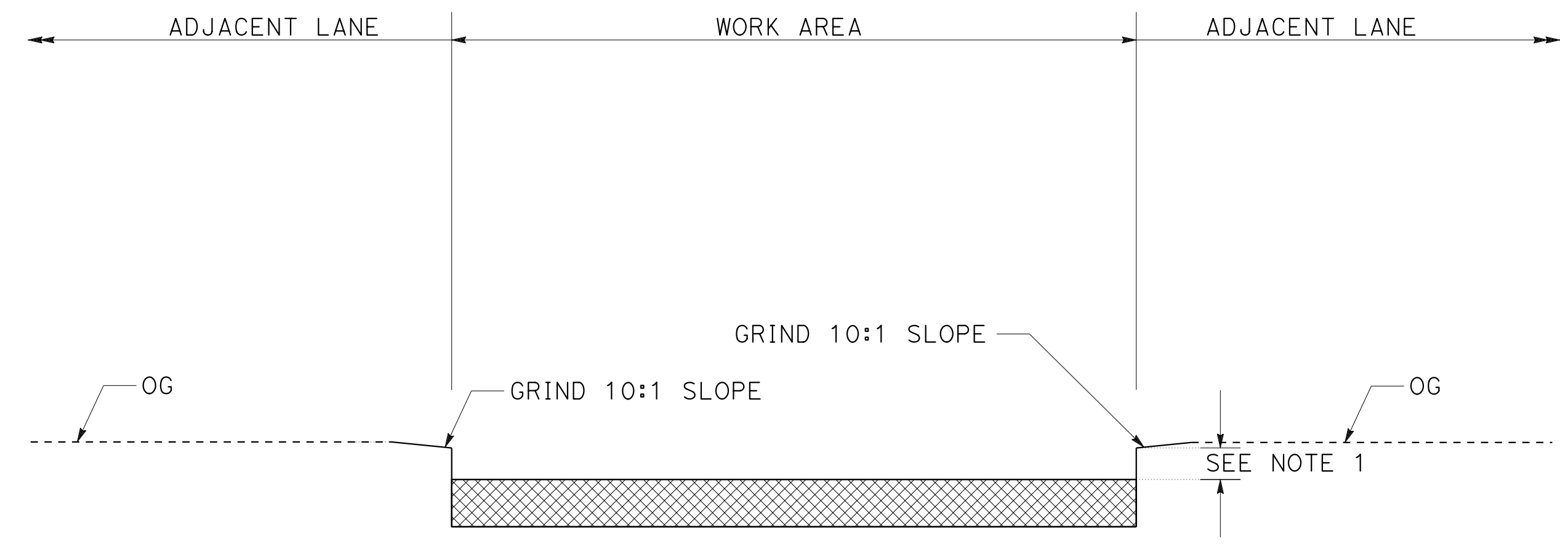
SAFETY EDGE DETAIL FOR HMA SECTIONS
