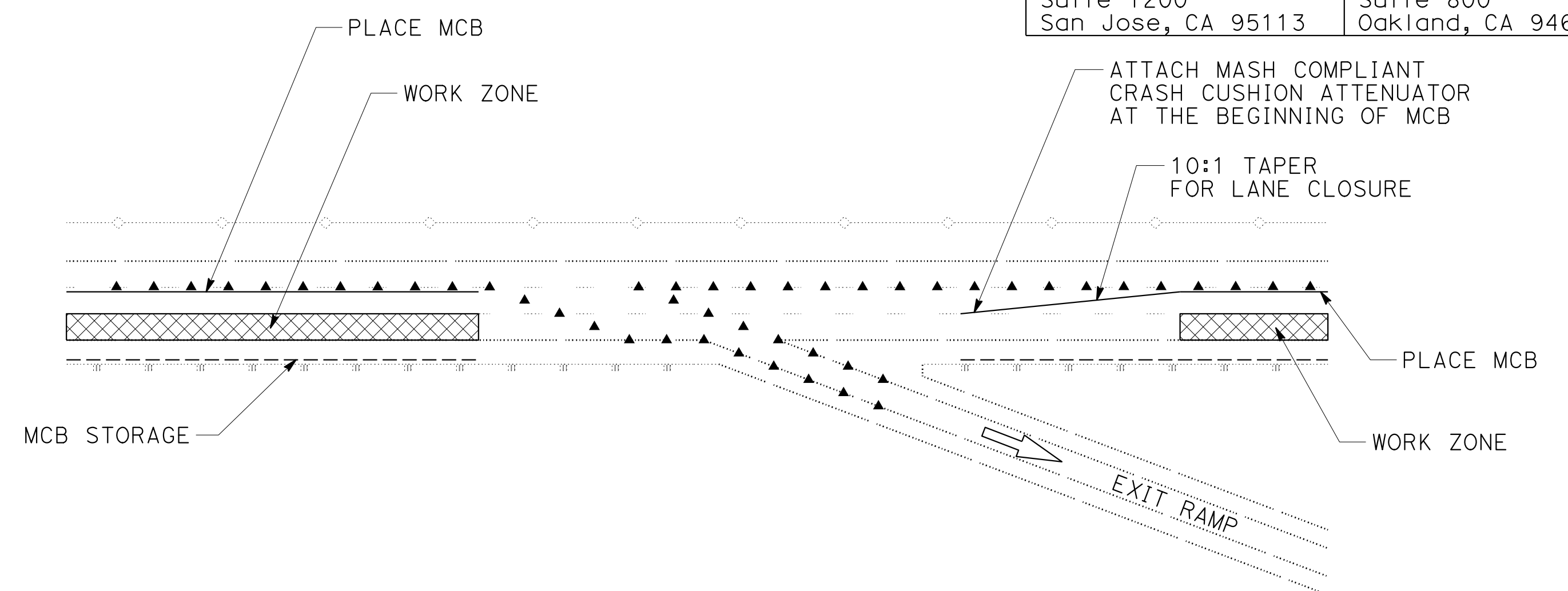
LANE CLOSURE AT EXIT RAMP (WORK AREA NEAR THE RAMP)
