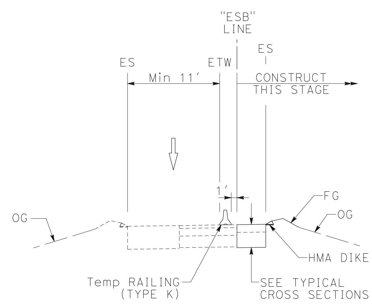
EB ROUTE 580 OFF RAMP TO SB ROUTE 680 SECTION E-E
