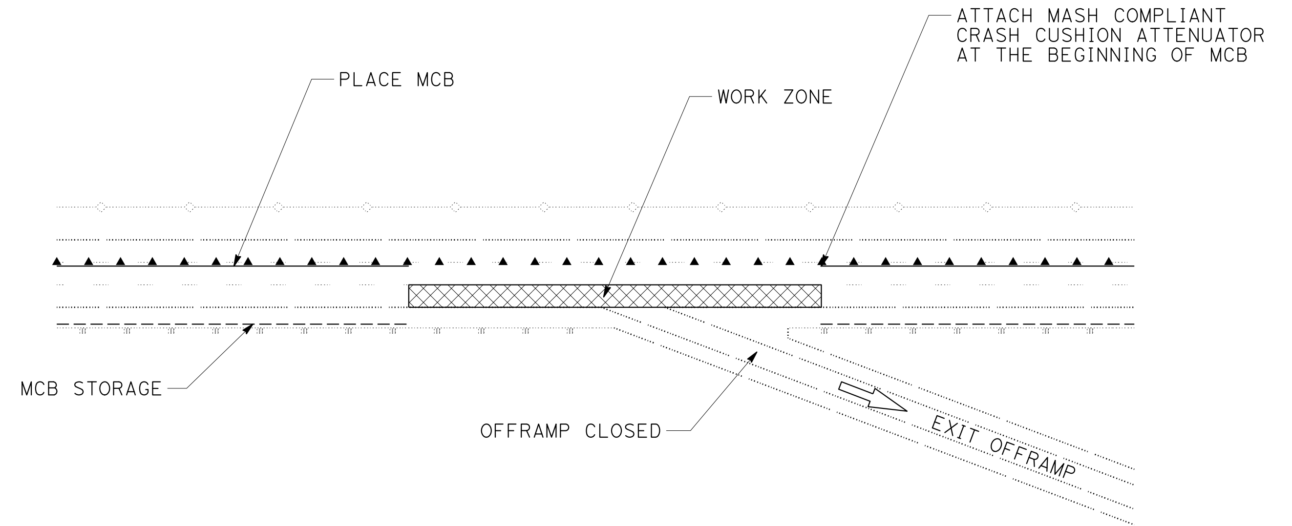
LANE CLOSURE AT EXIT RAMP (WORK AREA AT THE RAMP)
