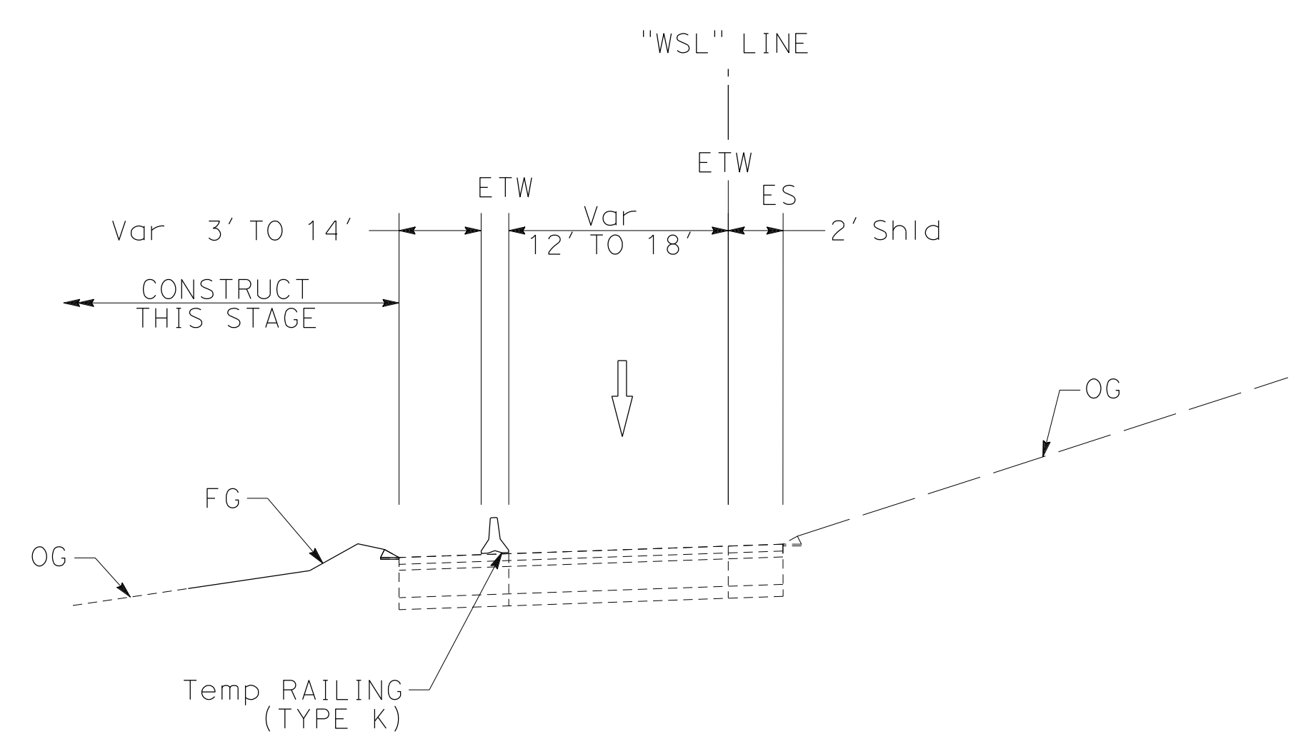
WB ROUTE 580 OFF RAMP TO SB ROUTE 680 SECTION F-F
