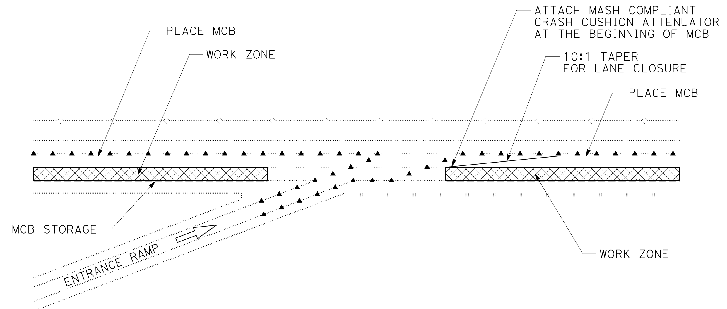
LANE CLOSURE AT ENTRANCE RAMP (WORK AREA NEAR THE RAMP)
