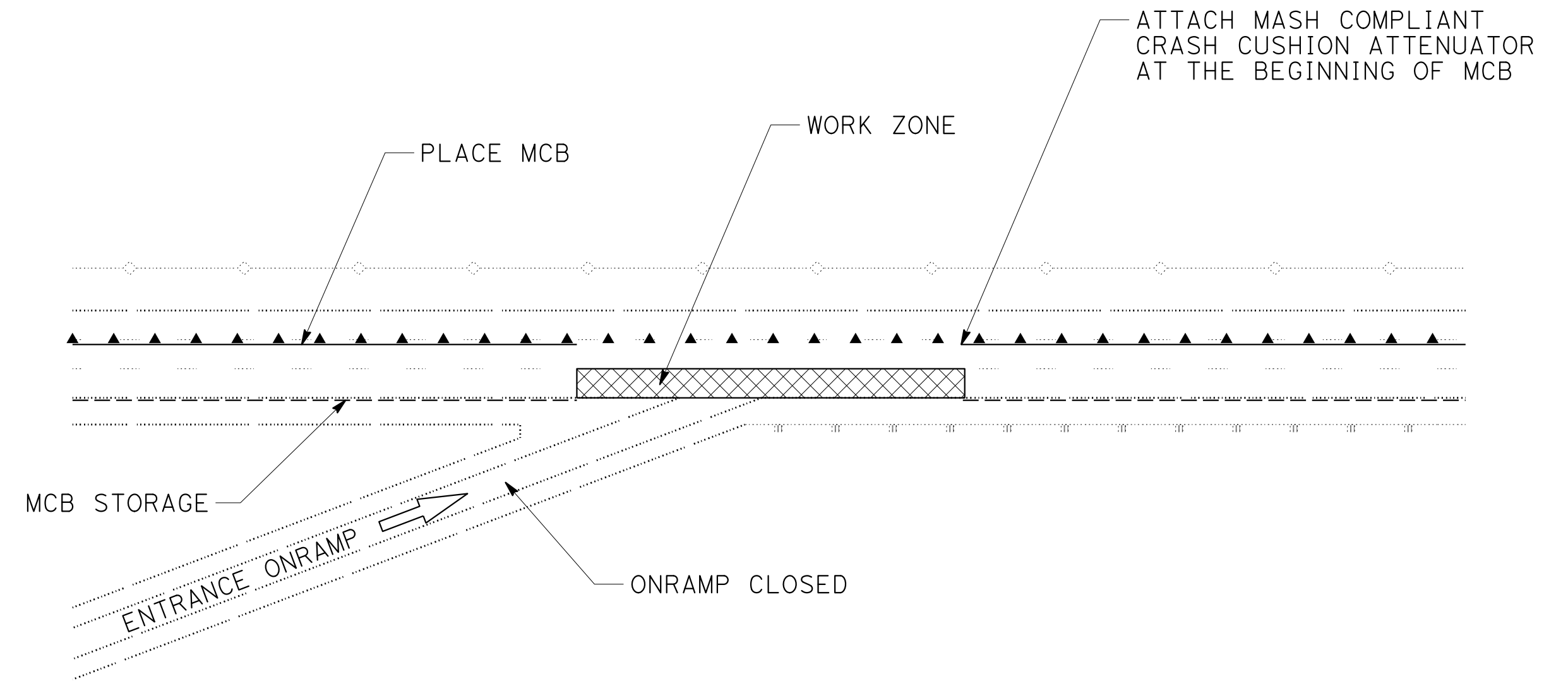
LANE CLOSURE AT ENTRANCE RAMP (WORK AREA AT THE RAMP)
