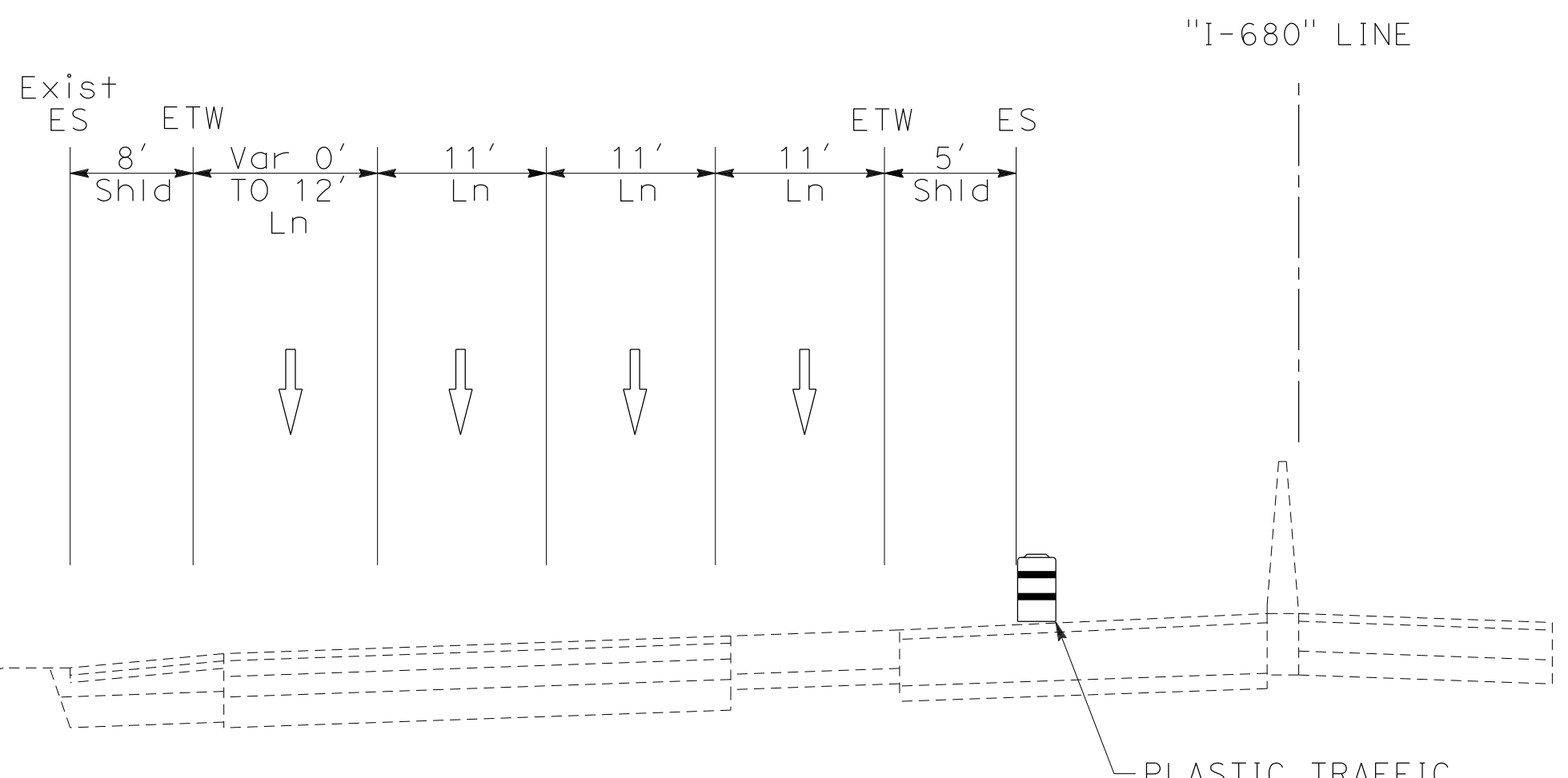
SOUTHBOUND ROUTE 680 SECTION L-L
