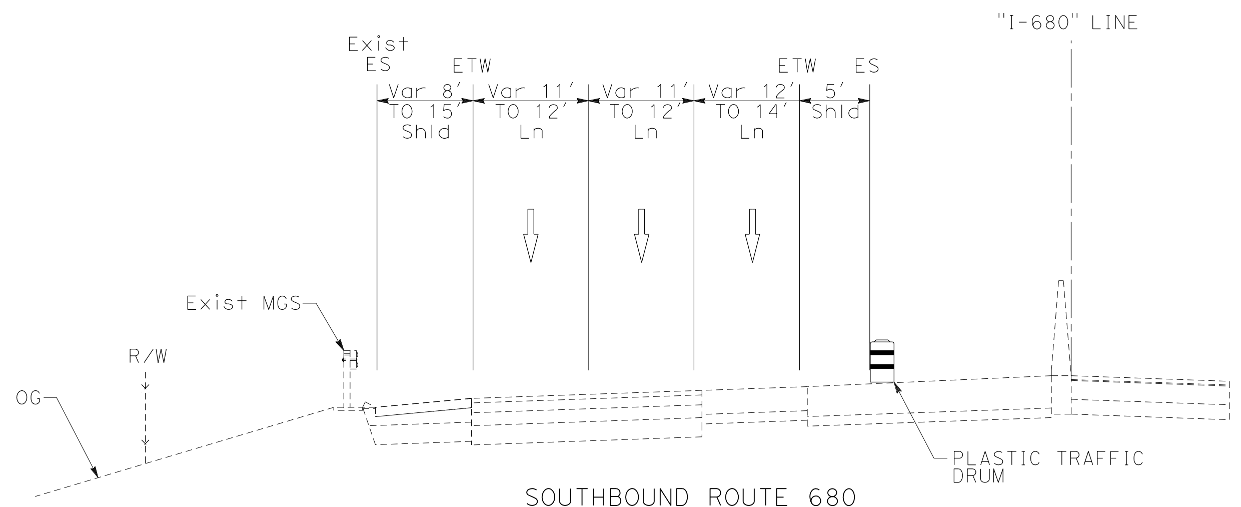
SOUTHBOUND ROUTE 680 SECTION O-O
