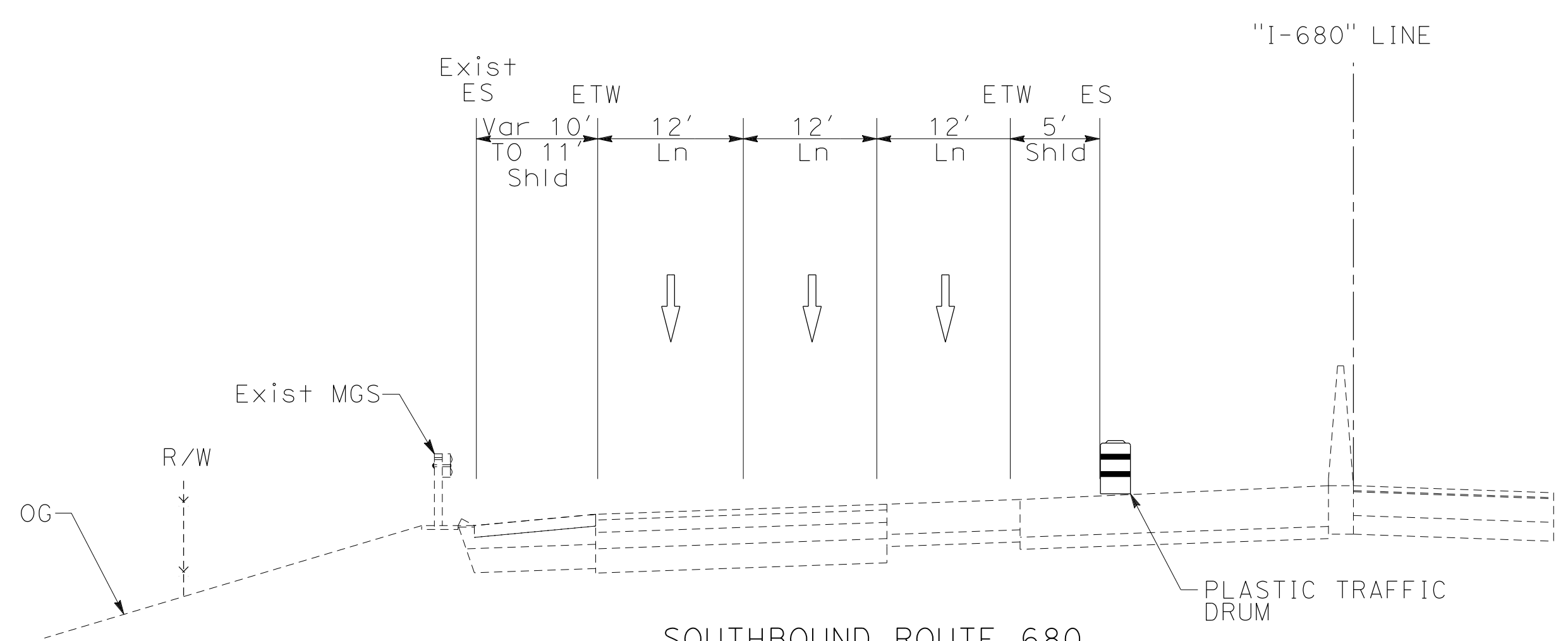
SOUTHBOUND ROUTE 680 SECTION N-N
