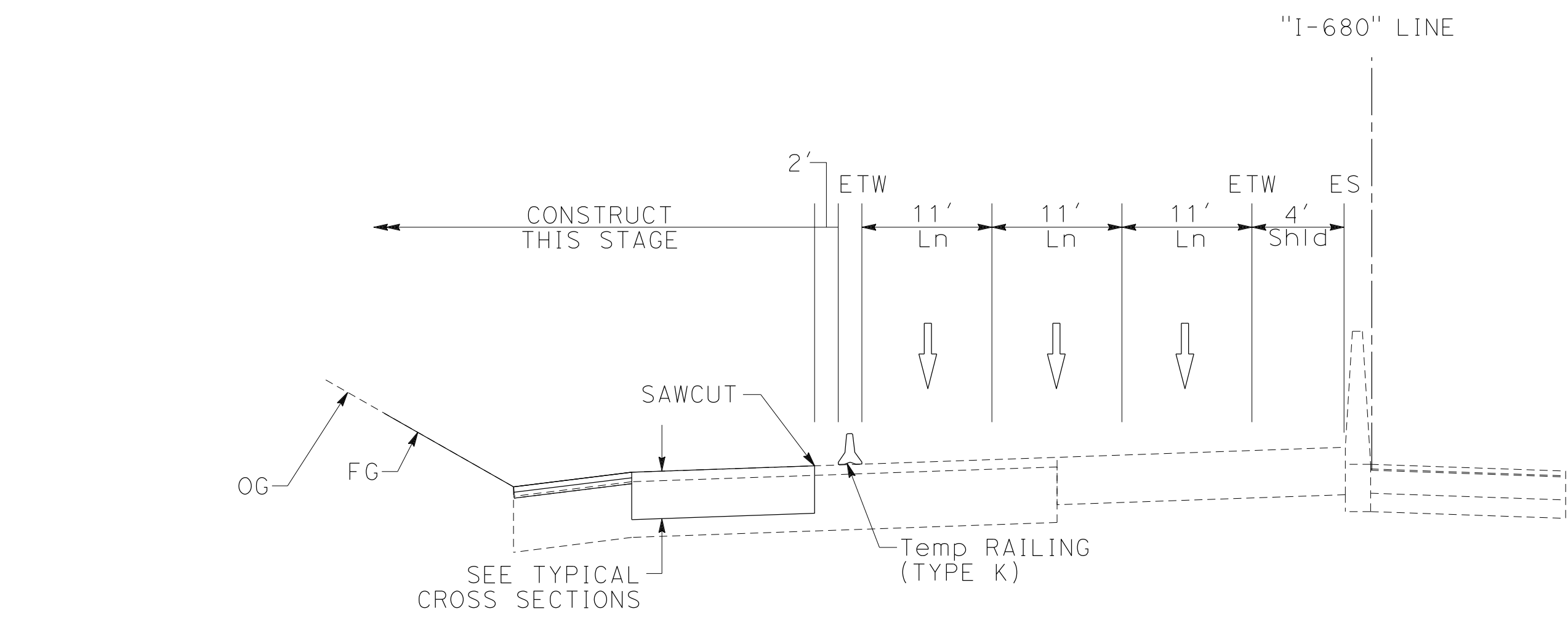
SOUTHBOUND ROUTE 680 SECTION K-K
