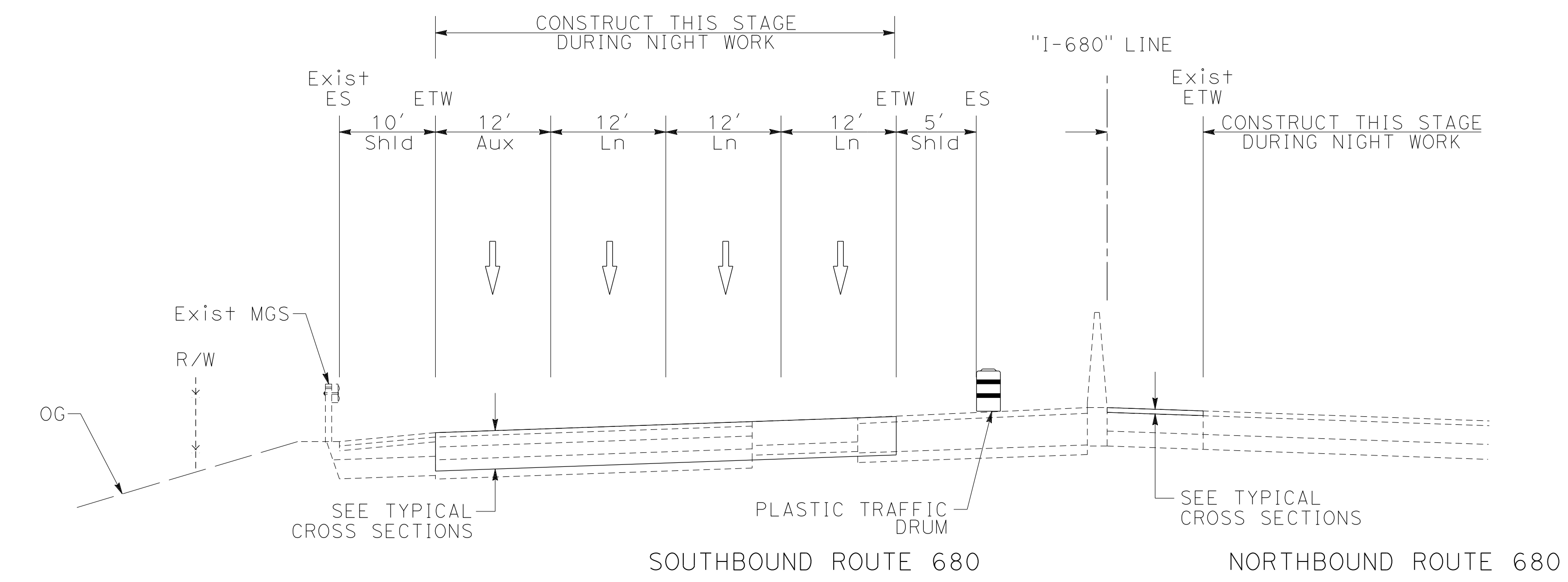
SECTION J-J
