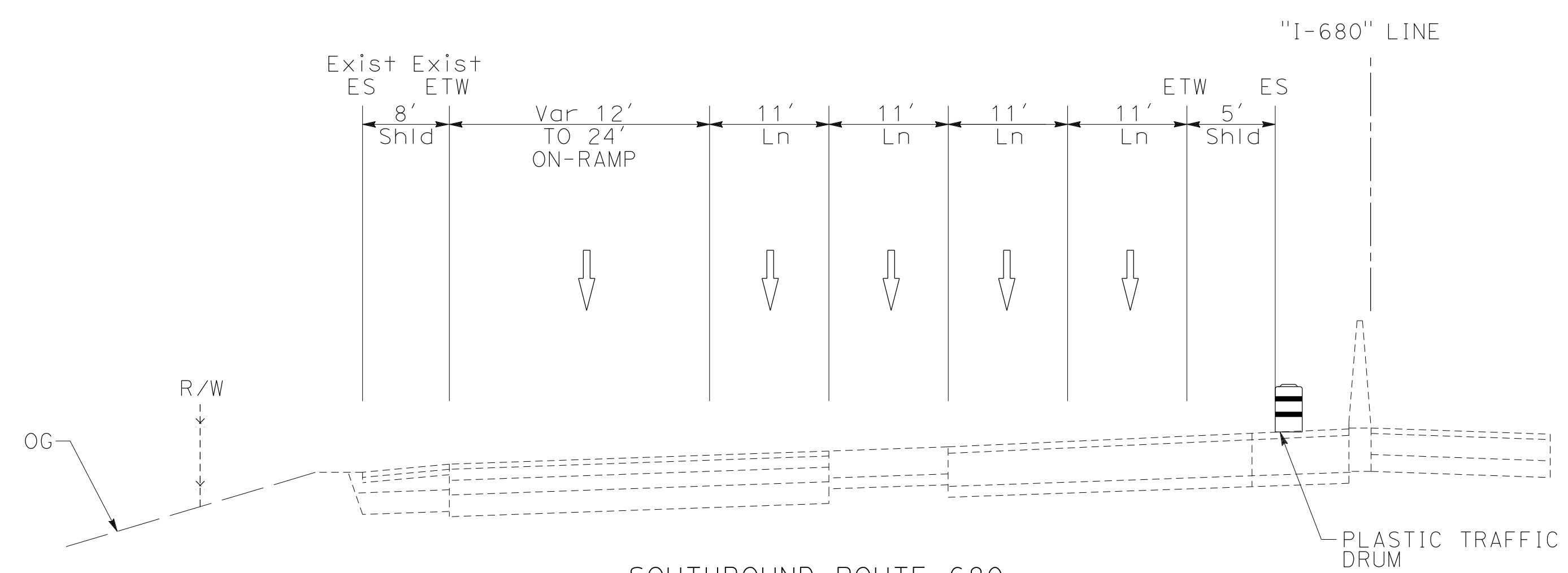
SOUTHBOUND ROUTE 680 SECTION O-O
