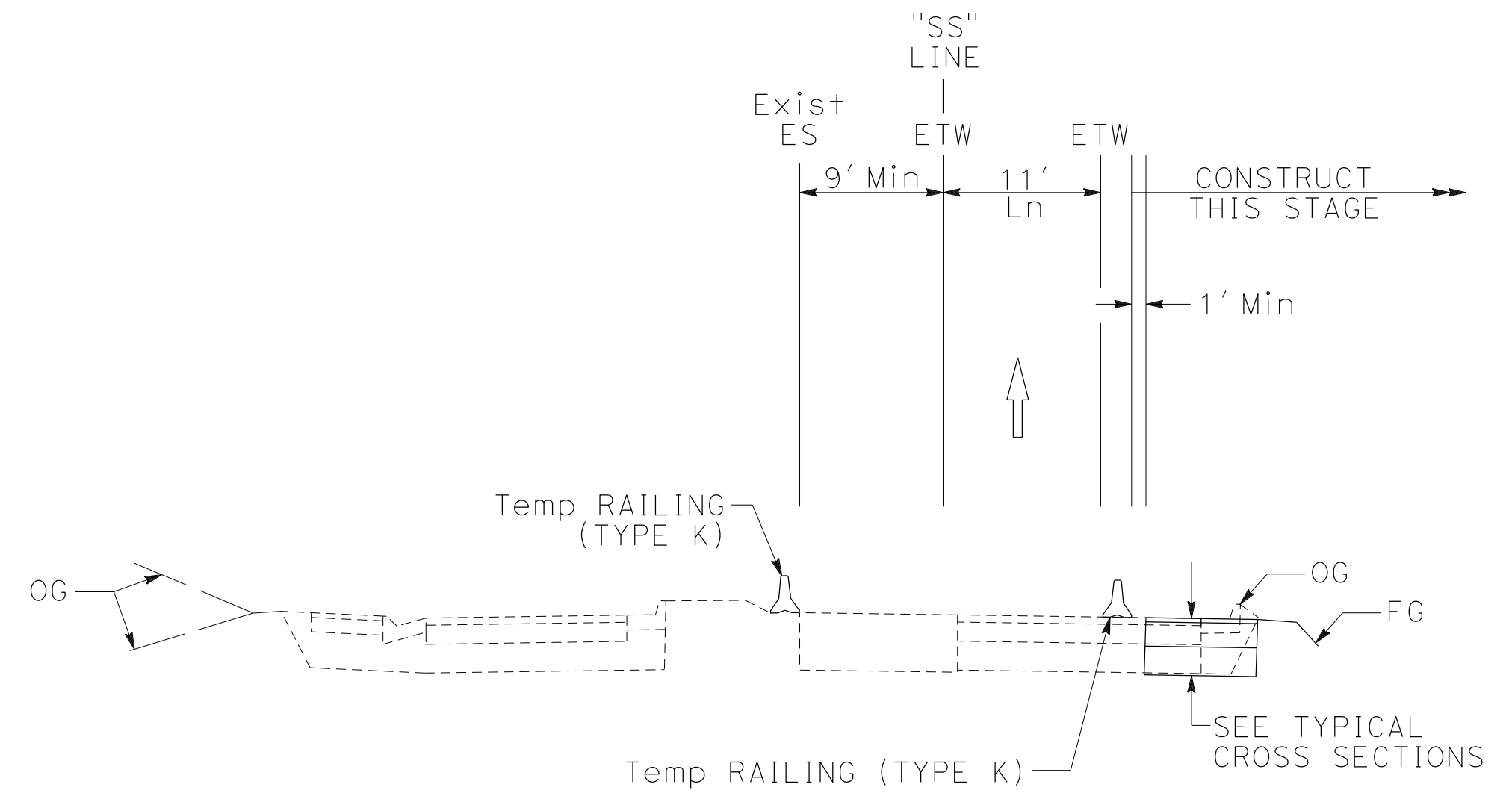
SB ROUTE 680 SUNOL BLVD ON RAMP SECTION G-G
