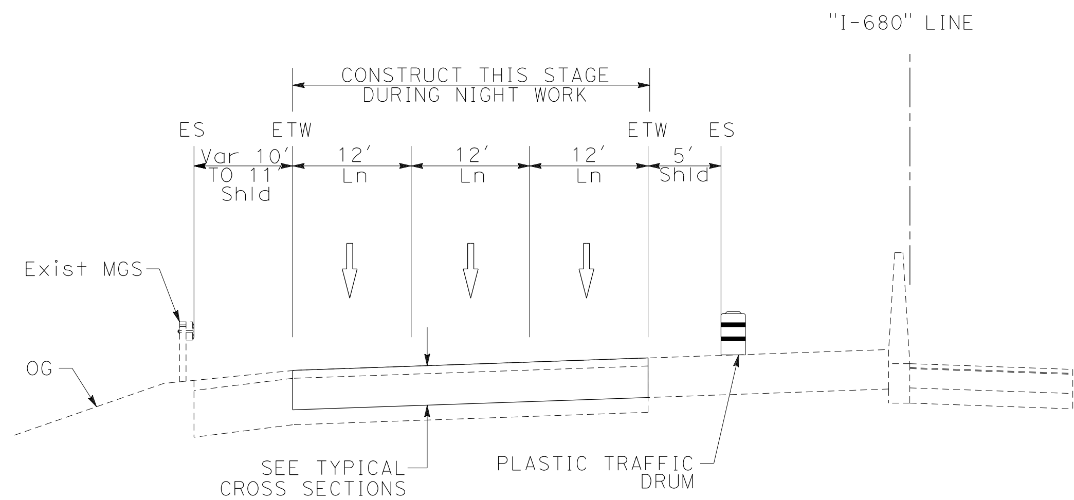
SOUTHBOUND ROUTE 680 SECTION F-F
