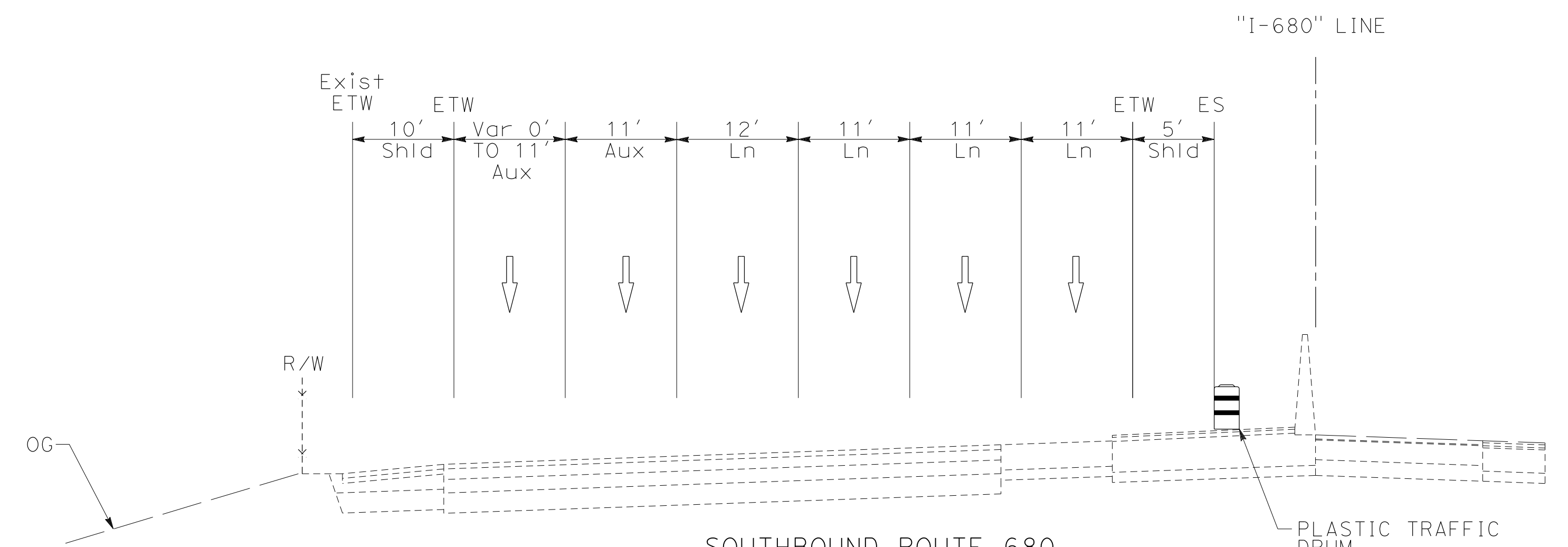
SOUTHBOUND ROUTE 680 SECTION N-N
