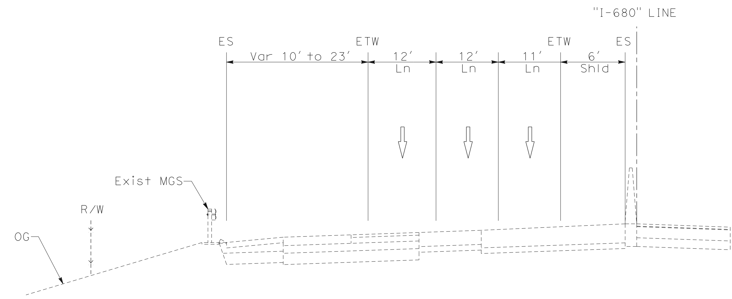
SOUTHBOUND ROUTE 680 SECTION L-L
