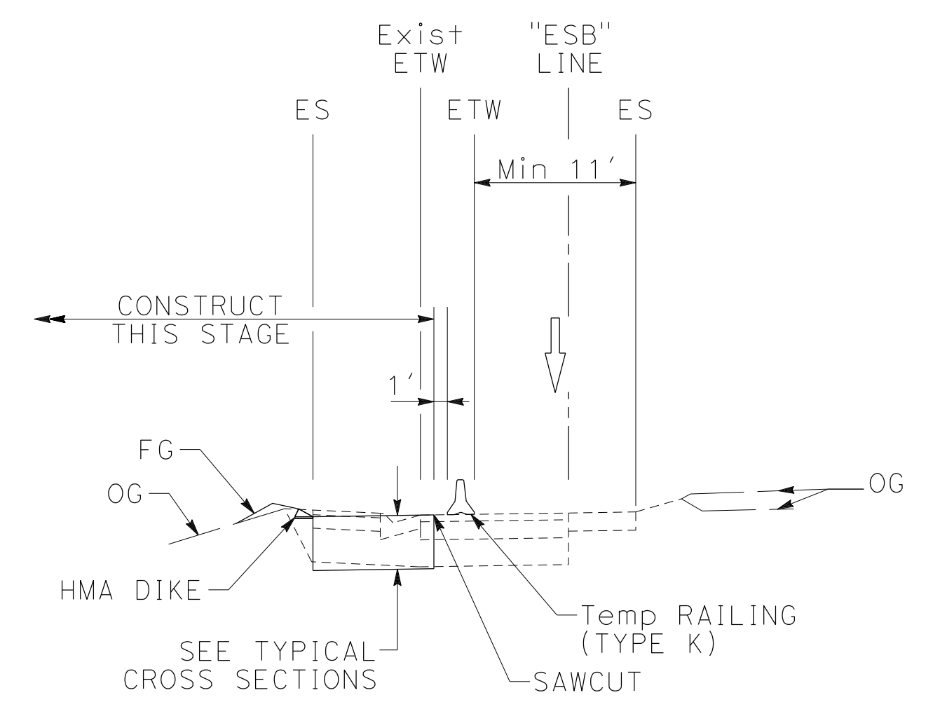
EB ROUTE 580 OFF RAMP TO SB ROUTE 680 SECTION K-K
