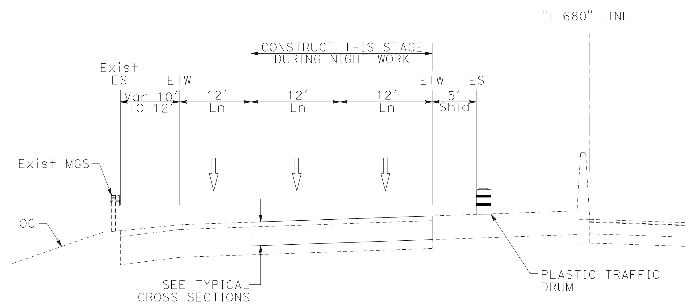
SOUTHBOUND ROUTE 680 SECTION G-G
