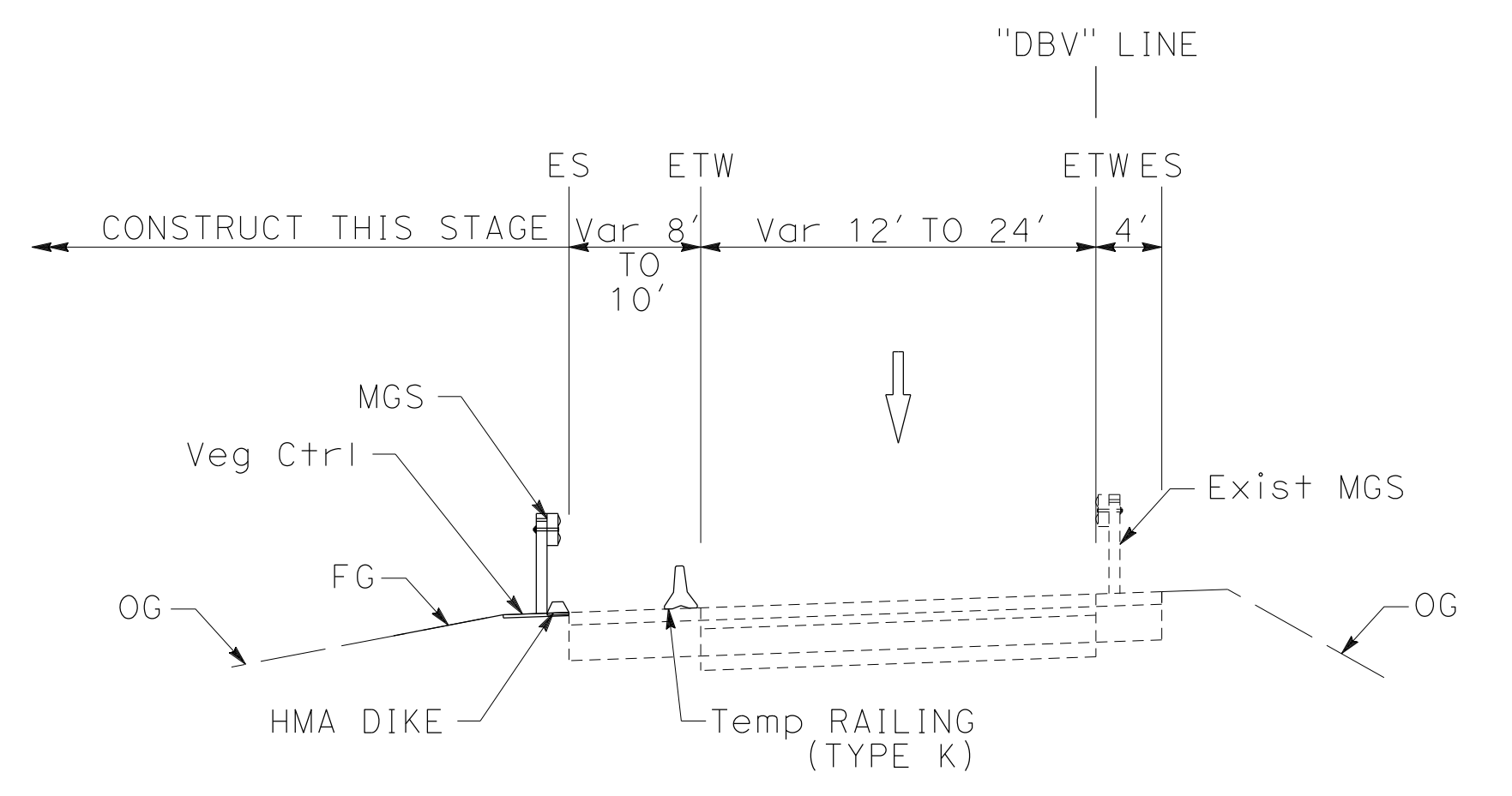
SB ROUTE 680 OFF RAMP TO AMADOR PLAZA Rd SECTION M-M
