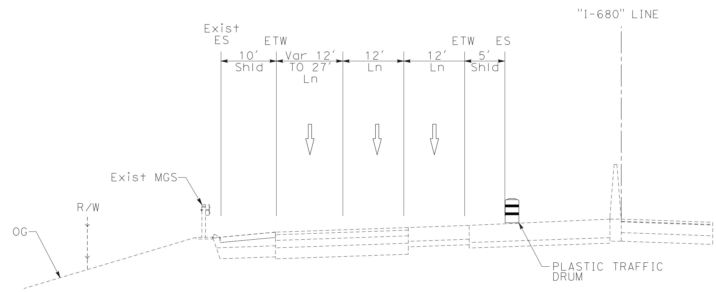
SOUTHBOUND ROUTE 680 SECTION M-M
