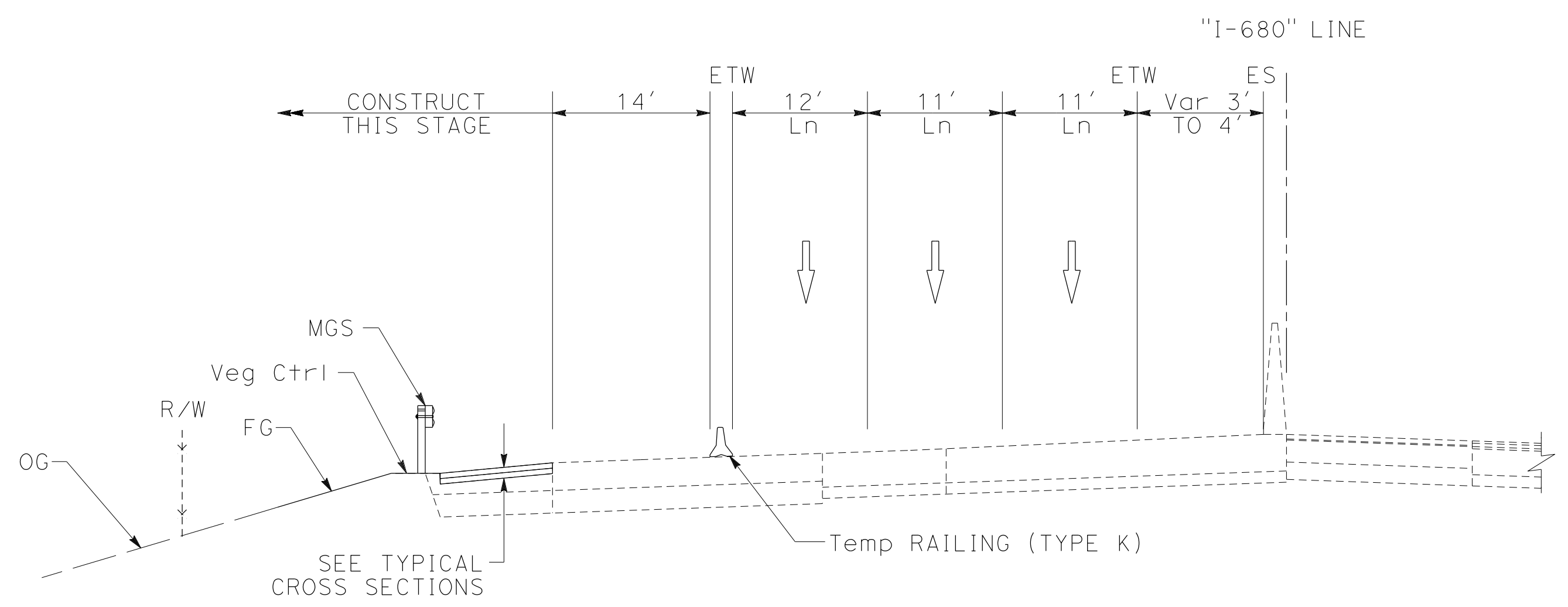
SOUTHBOUND ROUTE 680 SECTION F-F
