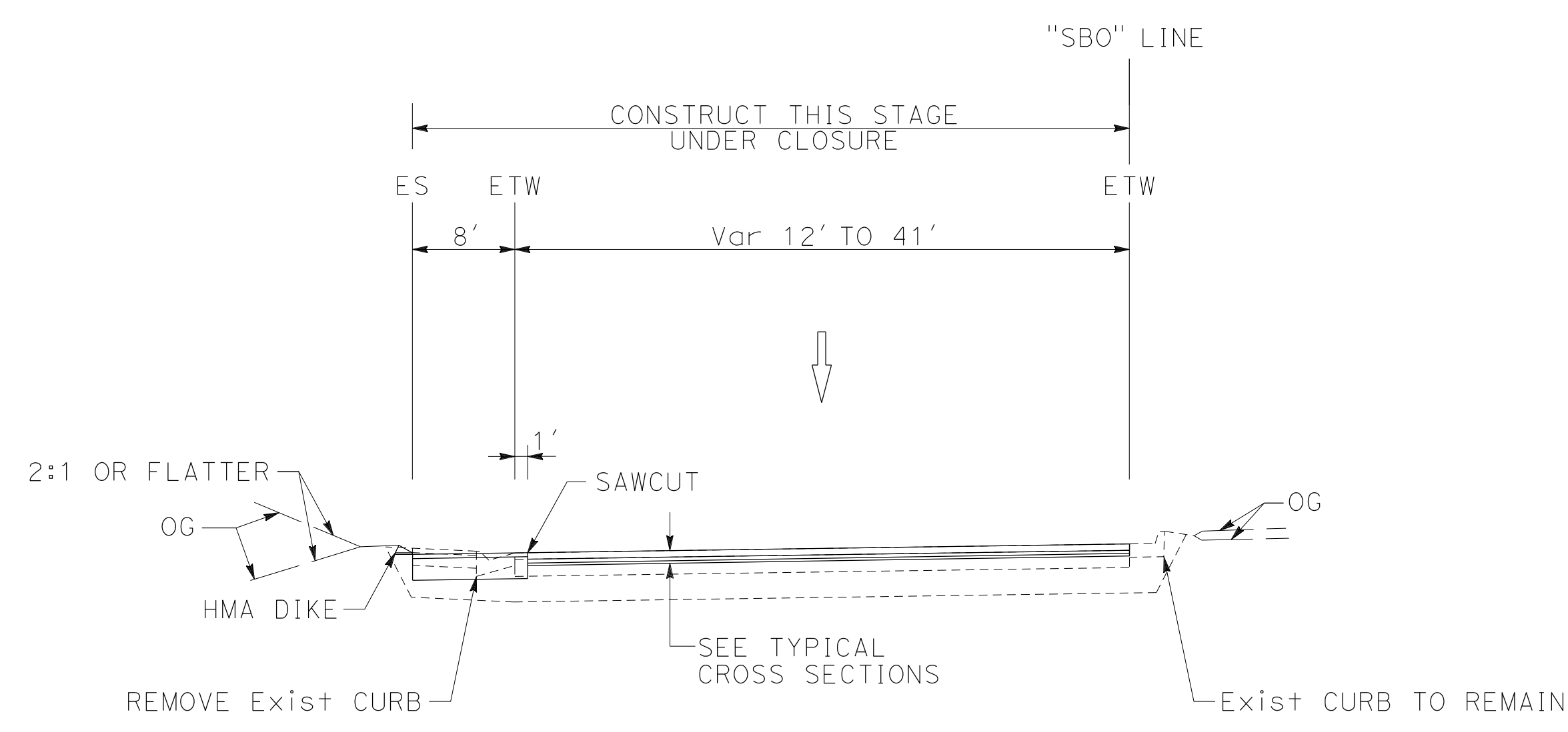
SB ROUTE 680 BERNAL AVE OFF RAMP SECTION H-H
