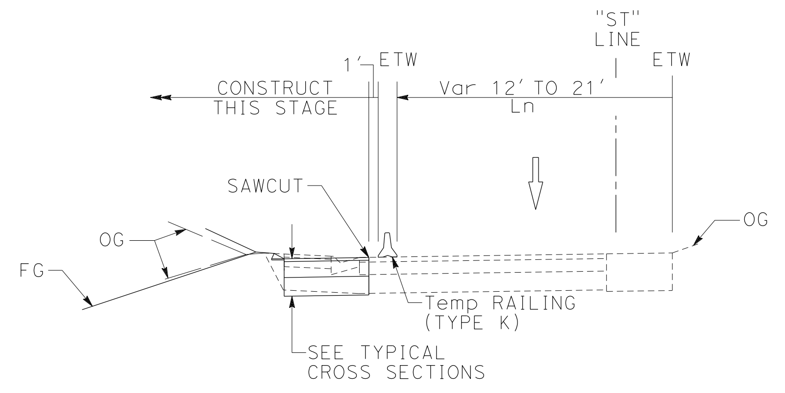
SB ROUTE 680 SUNOL BLVD OFF RAMP SECTION H-H
