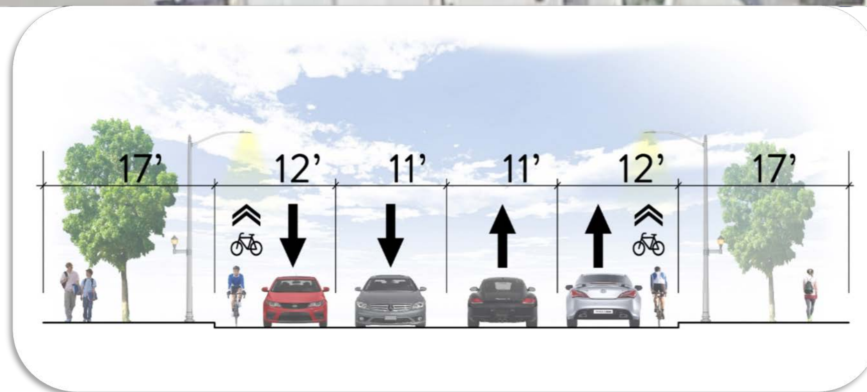
SECTION C-C
