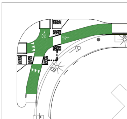
TYPICAL RAISED BIKEWAY AT INTERSECTION
