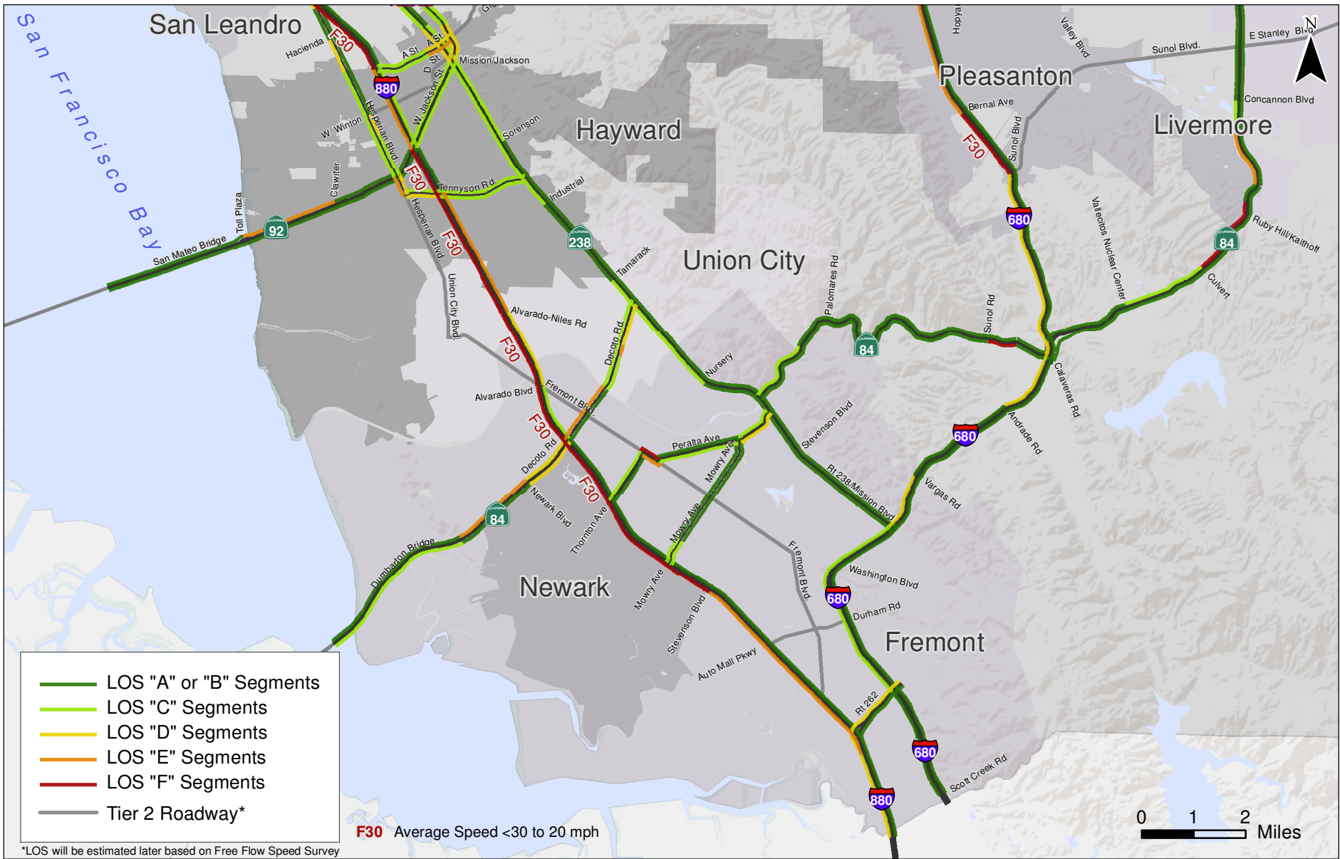
2012 AM Peak Period Level of Service Results Planning Area 3
