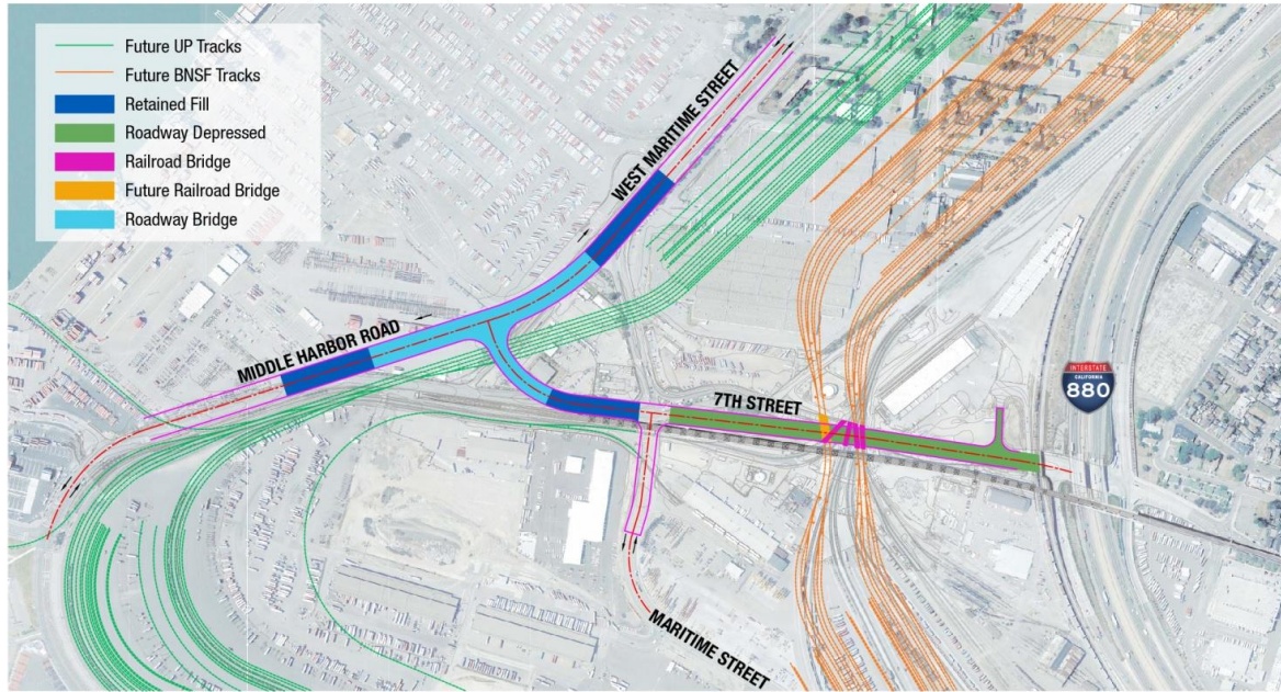
Figure 3.1 Preferred OHIT 7 th Street Grade Separation Alternative
