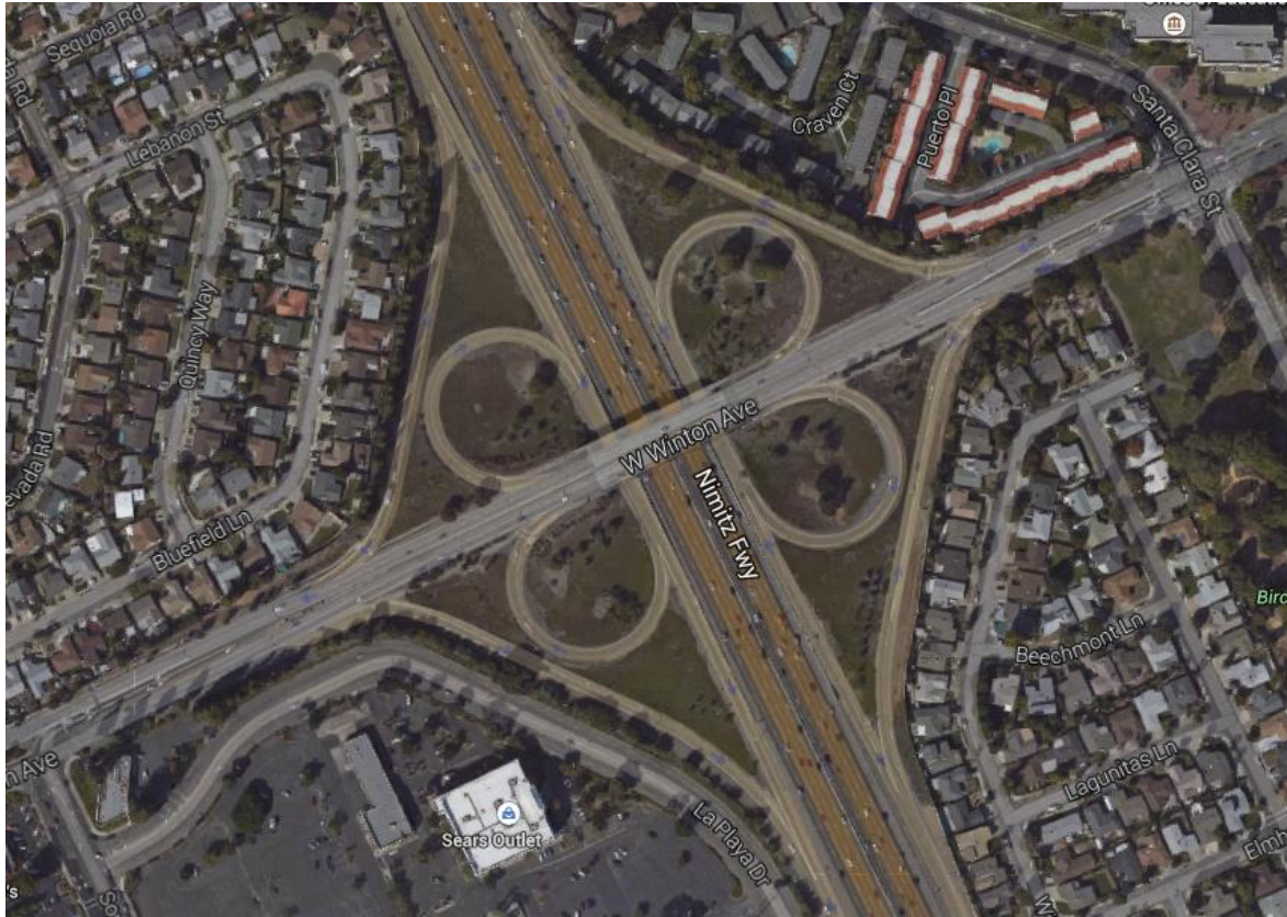
Figure 6.1 I-880/Winton Avenue Interchange Before
