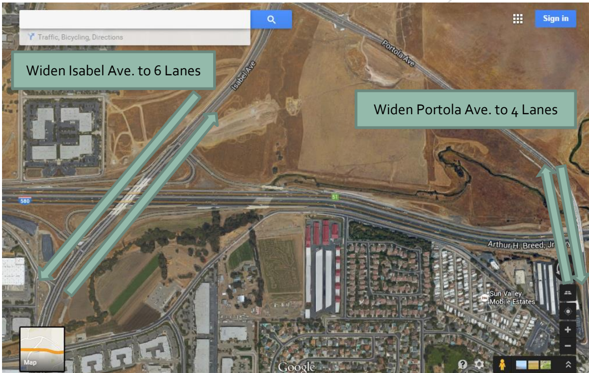
Figure 6.13 I-580/Isabel Avenue Interchange Phase 2 Project Location
