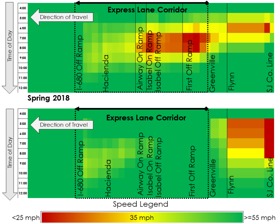
Figure 17: Westbound Bottlenecks and Queuing 2015 and 2018 across All Lanes Spring 2015
